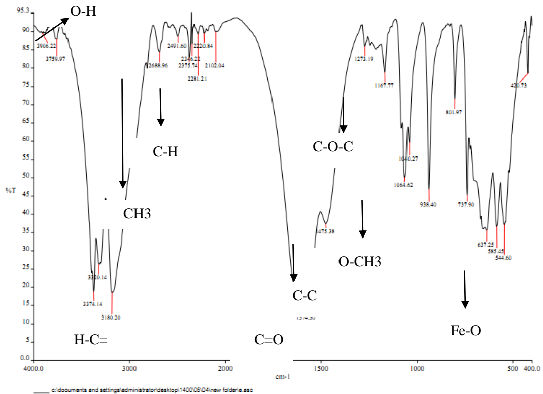
Fig. 1 FT-IR spectra of SNPsGQD@β-cyclotriacetal.
