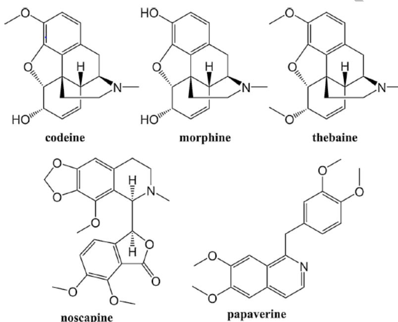
Fig. 3 Chemical structures of the Papaver alkaloids calculated in poppy
