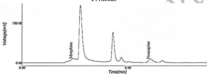
Fig. 5 The chromatograms of collected plant samples
