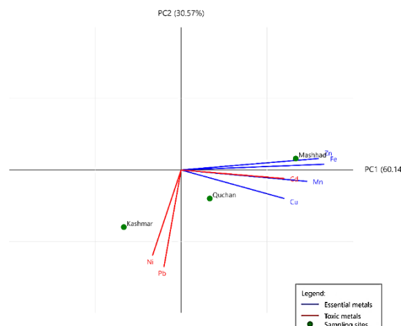
Fig. 1 PCA biplot of heavy metal relationships and market distribution patterns in lavender samples from Khorasan Razavi region, Iran. Loading vectors show the distribution of seven analyzed metals (Fe, Zn, Cu, Mn, Cd, Pb, Ni) across the first two principal components (PC1: 60.14%, PC2: 30.57%, total variance explained: 90.71%). Essential metals are shown in blue vectors, potentially toxic metals in red vectors, and market locations as green circles. The data represents mean values from 18 composite samples collected from three major medicinal plant markets ( n=6 per market).
