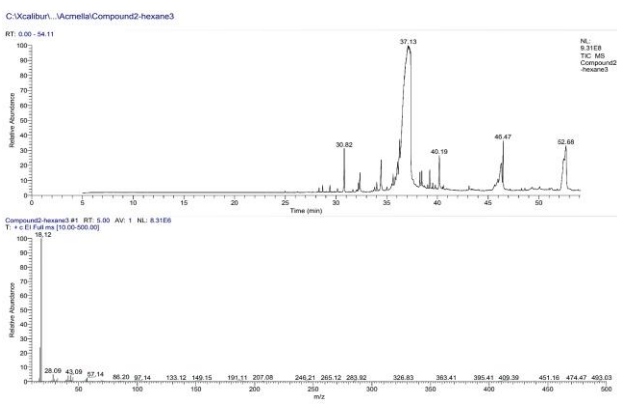
Fig. 6 GC-MS chromatogram and spectra of a compound isolated from A. oleracea . Structure of lup-20(29)-en-3-ol as generated from the NIST chemical library.
