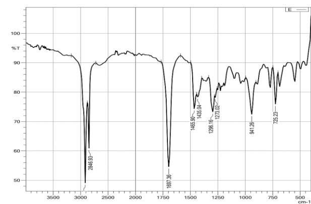
Fig. 5 FTIR spectra of a compound isolated from A. oleracea .
