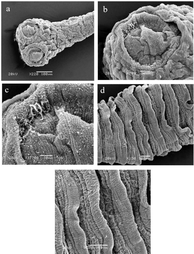
Fig. 8 Scanning electron micrographs of different body parts of poultry tapeworm treated with a compound isolated from A. oleracea . (a) Scolex and neck region showing rostellum (slight depression) at the tip and two oval suckers. (b) One sucker focussed to show removal of the tegument and the spines. (c) Magnification of the same sucker showing almost complete loss of the spines except for four of them (white fang-like structures) on the top. (d) The main body showing a chain of body segments, and the body surface is abnormally folded. (e) Enlarged view of the mature segment indicating heavy tegumental folds and several tissue debris and warts.
